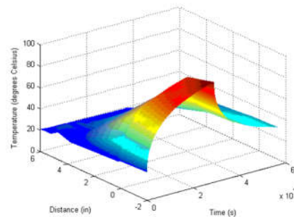
Fig. 6 PCM wall temperature time history versus location
